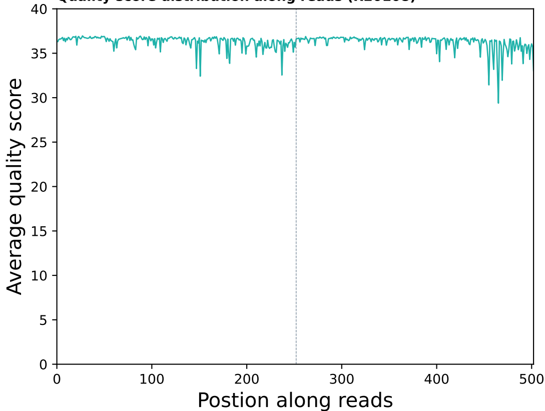
Quality score distribution along reads (R20108)
